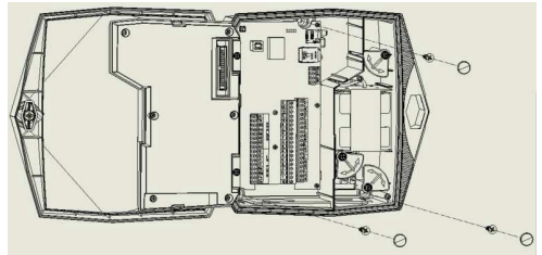
Figure 6: Inserting the Mounting Screws with Cover Caps
