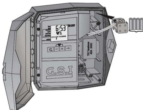
Figure 8: Battery Compartment Removed
